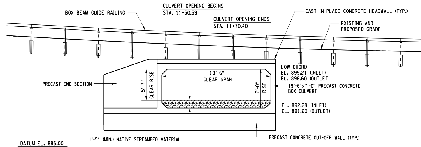
CULVERT ELEVATION
